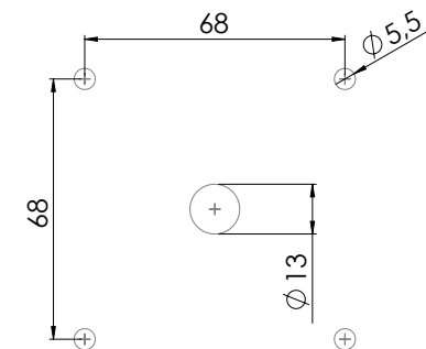
Bohrbild / Hole pattern
